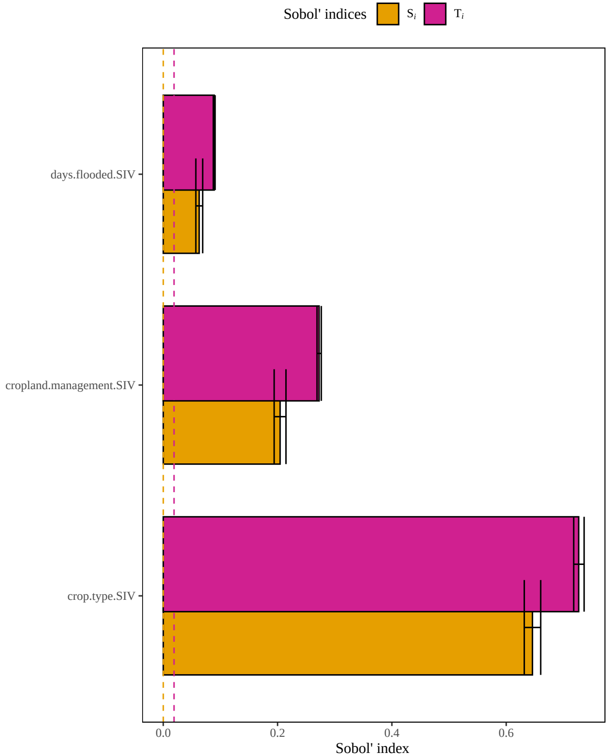
Figure 5. Results of a sensitivity analysis for the mallardCroplandSoy model based on a geometric mean structure. Dashed lines represent baseline numerical approximation error for S_i and T_i ( i.e. , dummy variables).
