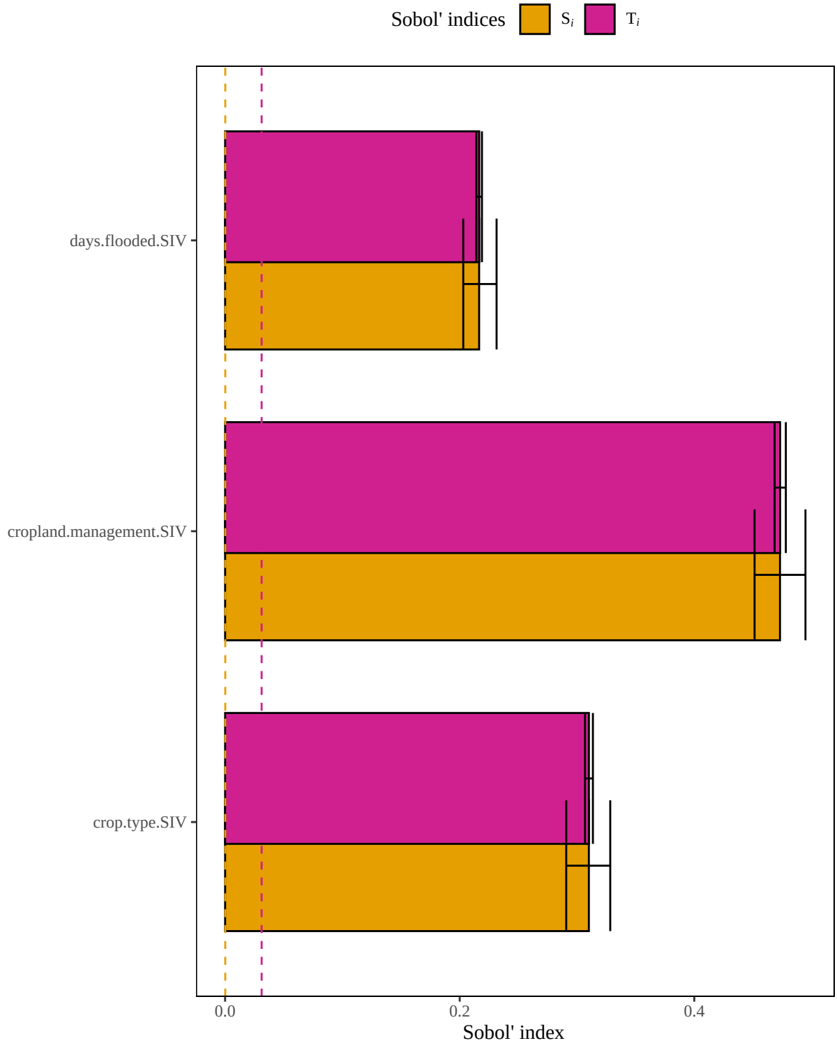
Figure 4. Results of a sensitivity analysis for the mallardCroplandSoy model based on an arithmetic mean structure. Dashed lines represent baseline numerical approximation error for S_i and T_i ( i.e. , dummy variables).
